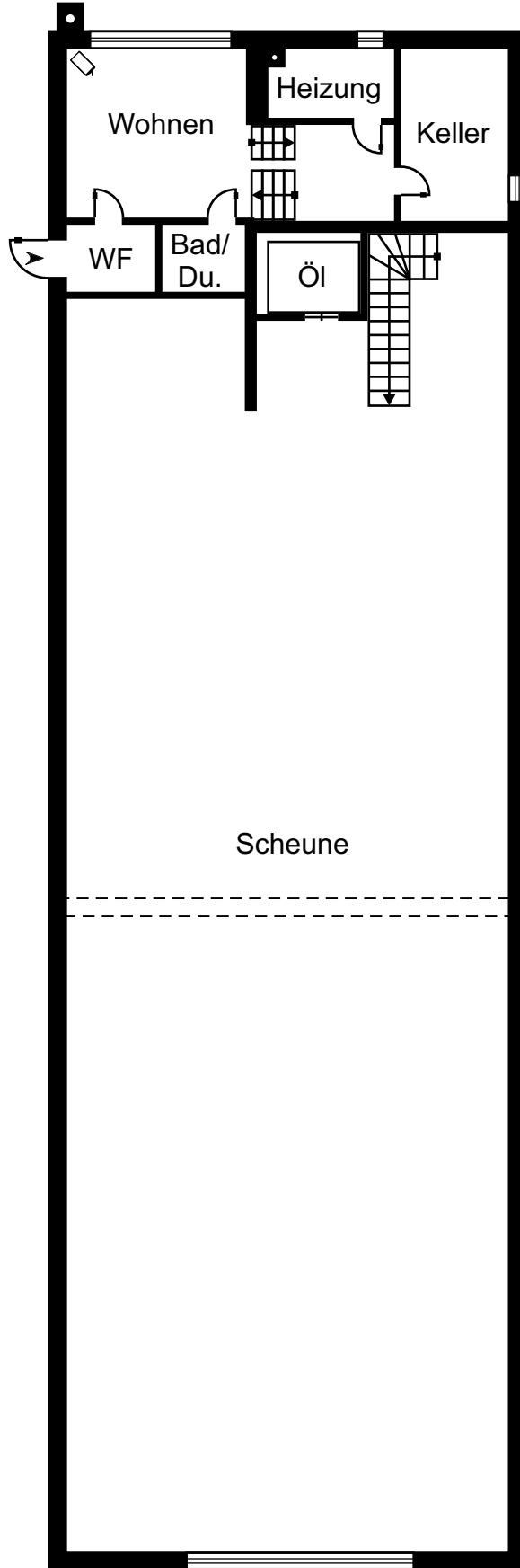
MB 22028 Erdgeschoss-Scheune
